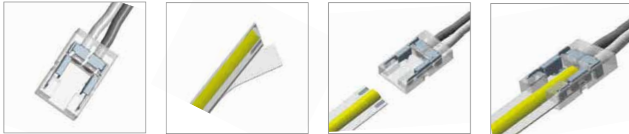
LW-A-SW-2 PCB width: 8/10mm Color: Single color
